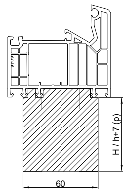
VEKA 82 NV030
