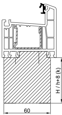
REHAU BRILLIANT NV026
