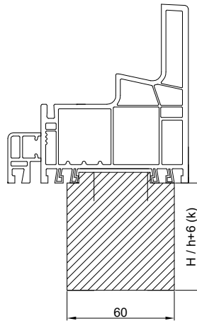
GEALAN KUBUS NV023
