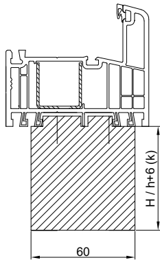
GEALAN S9000 NV022
