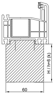
GEALAN S8000 NV021
