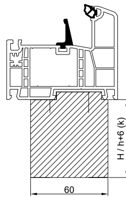
REHAU GENE0 NV028
